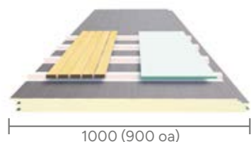
CP Business Line ALPHA-AR FX CARRIER 120 mm Uniek FX brandwerend getest carriersysteem EI30
